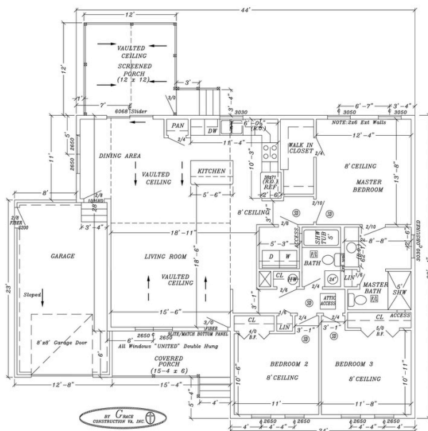
"THE BAYSIDE" (2025CODE) 1436 sq. ft. Total Living Space 236 sq. ft. Covered Porches 280 sq. ft. Garage
