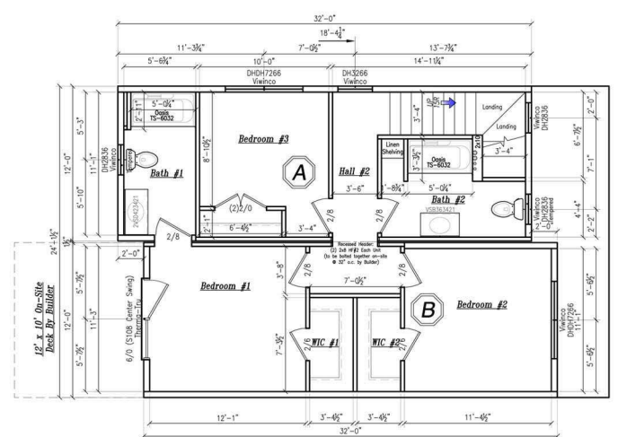
Second Floor Plan SCALE: 3/16" = 1'-0"
