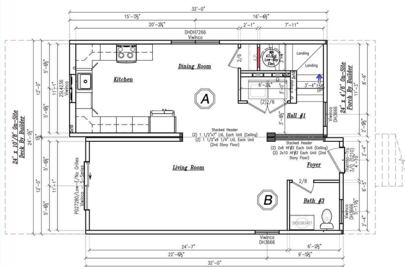
First Floor Plan SCALE: 3/16" = 1'-0"
